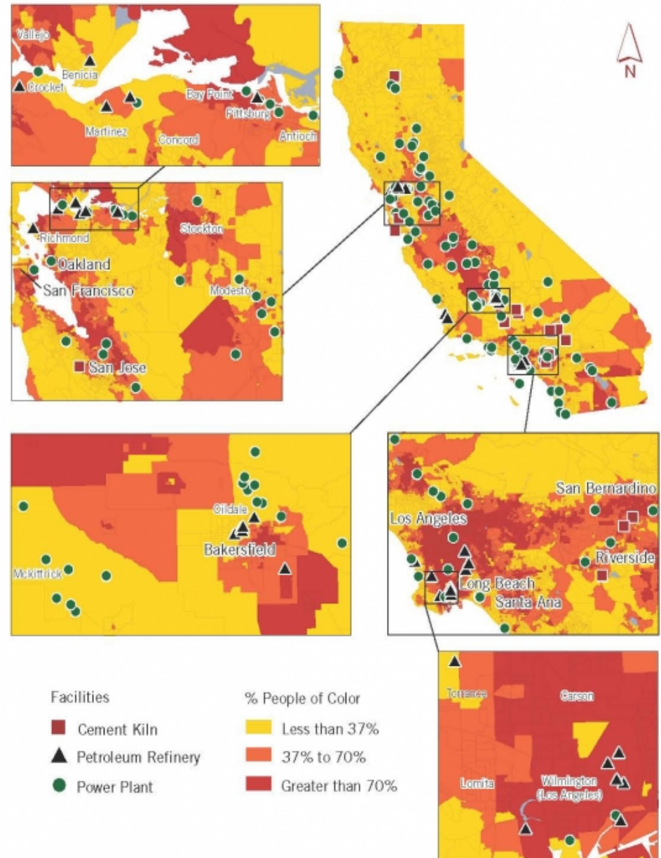
Figure 1: Major GHG-Emitting Facilities in California
